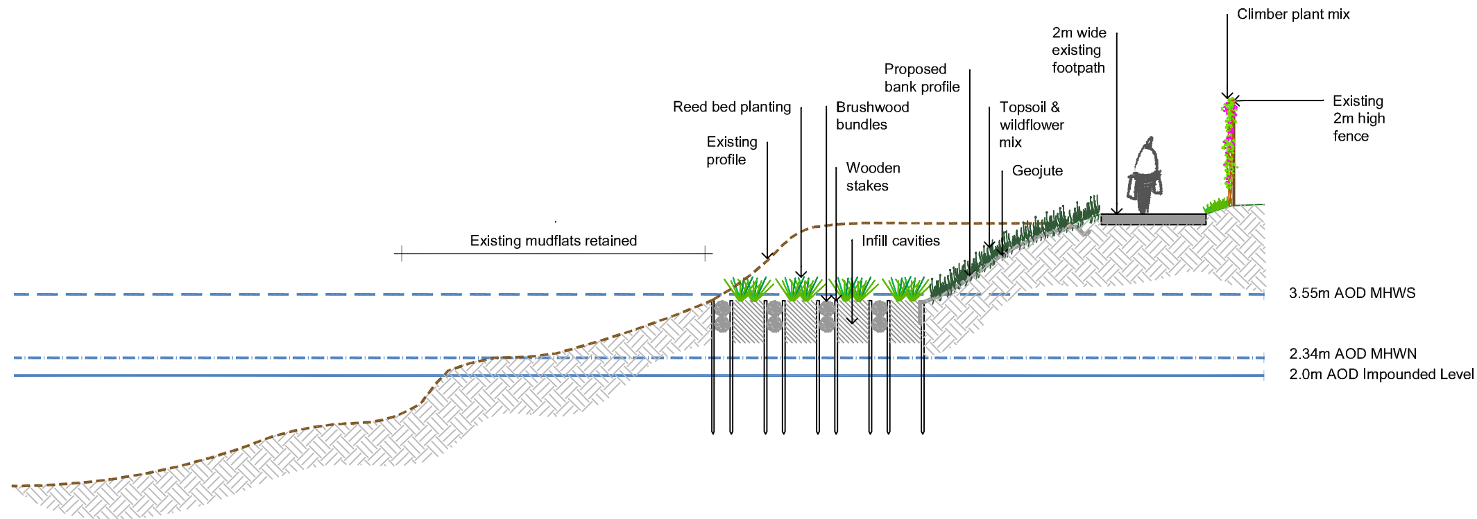
Section A-A - East Bank Reach 3
